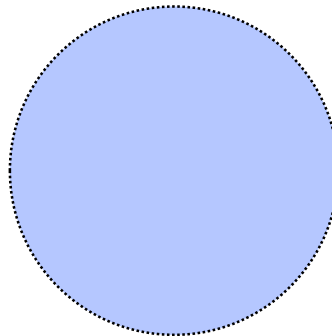
Sirius B
