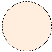
Proxima Centauri
